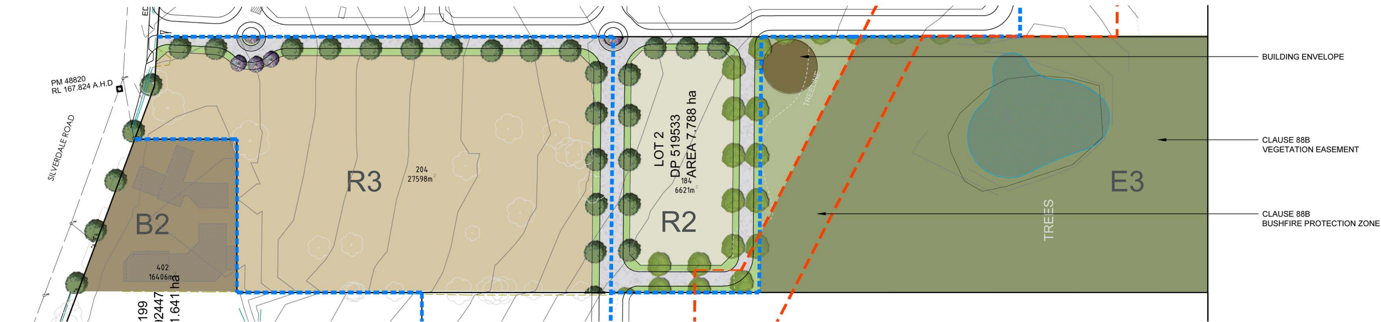
LOT 2 - DP19533 & LOT 199 DP1092447 - PLAN 1:1250
